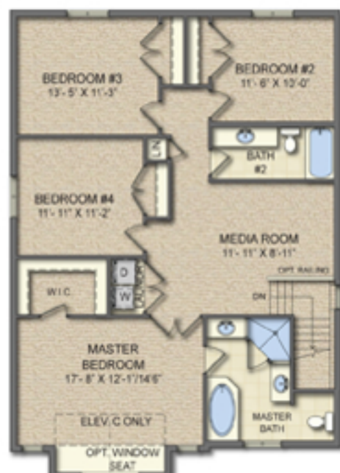
Alt. Second Floor (4 Bedroom) (Elevation A, B & C 1,304 sq.ft.)
