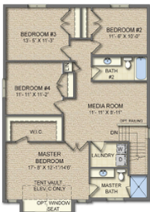
Second Floor (4 Bedroom) (Elevation A, B & C 1,304 sq.ft.)
